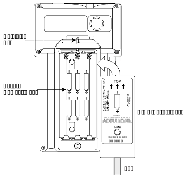
Figure 2-7: Changing Batteries
